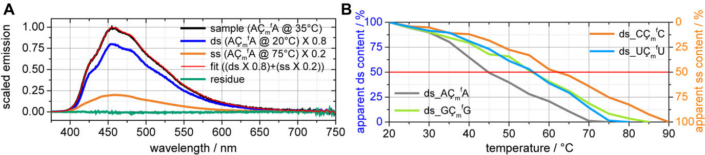
Figure 5. (A) Spectrally resolved melting analysis of the emission spectra of ds\_AC_m^fA at 35°C. (B) Temperature dependence of the double-to-single-stranded-content of the four labeled double-stranded samples, determined by spectrally resolved melting analysis.
