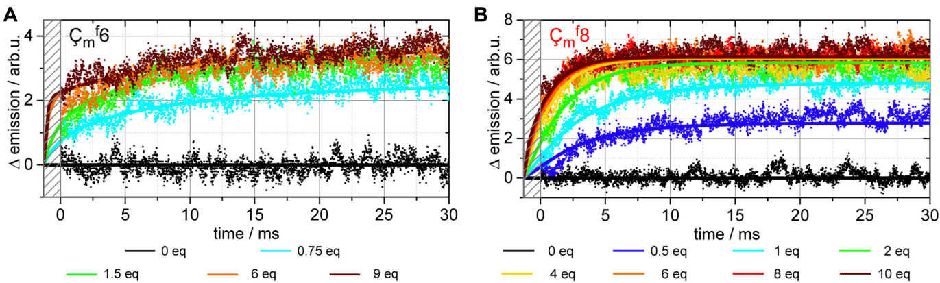
Figure 11. (A) Transient fluorescence signals after stopped-flow mixing of (A) 2.7 μM C_m^f6 and (B) 4 μM C_m^f8 with different concentrations of neomycin (indicated as equivalents of the aptamer concentration). The data are shown as points while the fits for a two-step model are displayed as solid lines.
