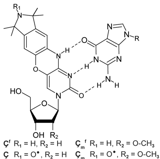
Figure 2. \text{C} , \text{C}_m^f , \text{C}_m and \text{C}_m^f base paired with guanine.
