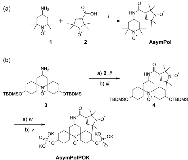
Scheme 1. (a) Synthesis of AsymPol (337 g mol −1 ) a ; (b) Synthesis of AsymPolPOK (765 g mol −1 ) b
