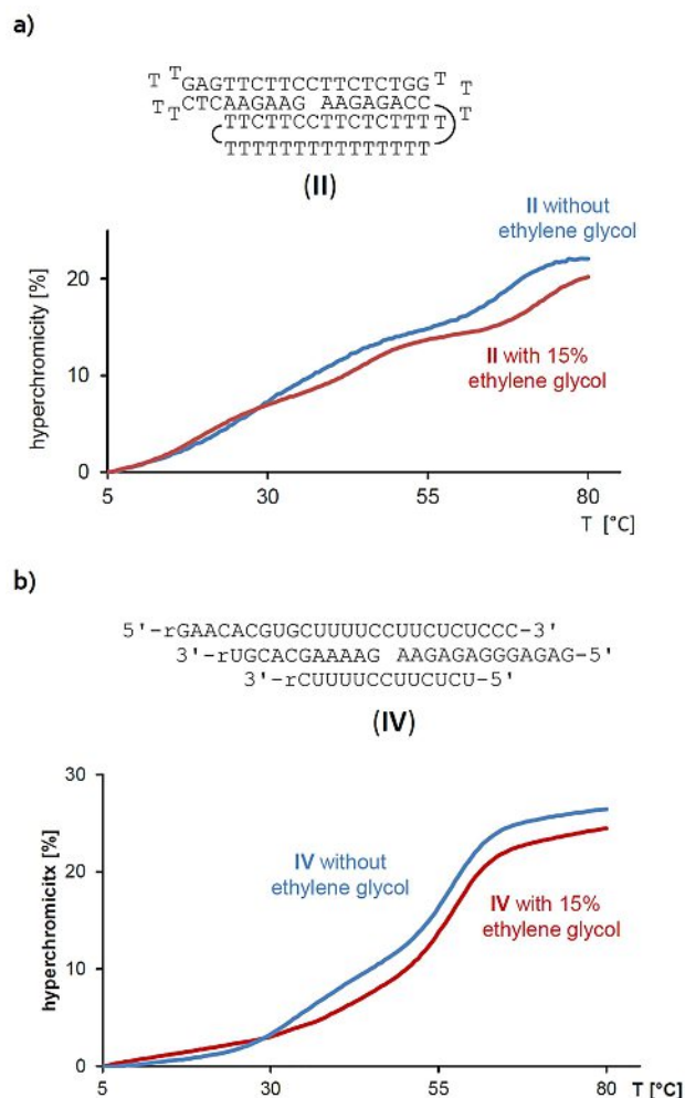
Figure 3. UV-melting curves of a) triplex DNA motif II , or b) RNA motif IV . Conditions: 1 \mu M strands in lithium phosphate buffer (10 mM, 150 mM NaCl, pH 6.0), with or without 15% ethylene glycol as co-solvent.
