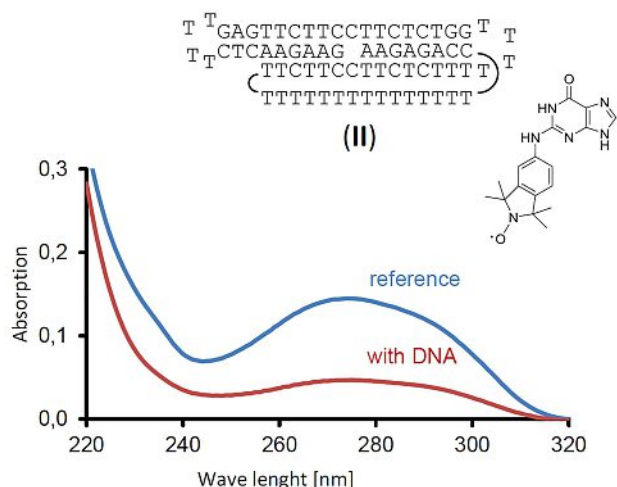
Figure 4. Absorption spectra of a solution of spin label Ĝ , either incubated with DNA motif II or by itself, after being subjected to filtration with a molecular weight cut-off of 3 kDa. Conditions: 9 \mu\text{M} Ĝ with or without 9 \mu\text{M} DNA motif II , 10 mM lithium phosphate buffer, pH 6, 150 mM NaCl, with 15% ethylene glycol as co-solvent, after filtration at 4 °C.
