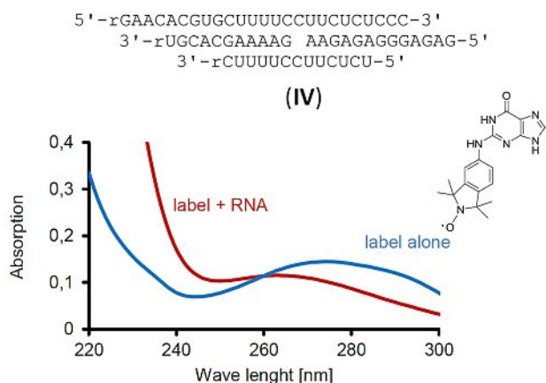
Figure 5. Absorption spectra of solutions of spin label Ĝ with or without intermolecular RNA motif IV , after filtration with a molecular weight cut-off of 3 kDa. Conditions: 9 \mu\text{M} Ĝ with or without 9 \mu\text{M} IV , 10 mM lithium phosphate buffer, pH 6, 150 mM NaCl, with 15% ethylene glycol, with filtration at 4 °C.
